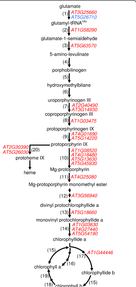
Figure 12 Changes in gene expression in chlorophyll biosynthesis of the glu1-2 mutant leaves. Schematic representation of chlorophyll biosynthesis and the genes showing different expression levels in glu1-2 leaves. Gene IDs indicated in blue are upregulated whereas those indicated in red are downregulated. Enzymes: (1) glutamate-tRNA ligase, (2) glutamyl-tRNA reductase, (3) glutamate-1-semialdehyde 2,1-aminomutase, (4) porphobilinogen synthase, (5) hydroxymethylbilane synthase, (6) uroporphyrinogen-III synthase, (7) uroporphyrinogen decarboxylase, (8) coproporphyrinogen oxidase, (9) protoporphyrinogen oxidase, (10) magnesium chelatase, (11) magnesium protoporphyrin IX methyltransferase, (12) magnesium protoporphyrin IX monomethyl ester cyclase, (13) 3,8-divinyl protochlorophyllide 8-vinyl reductase, (14) protochlorophyllide oxidoreductase, (15) chlorophyll synthase, (16) geranylgeranyl reductase, (17) chlorophyllide a oxygenase, (18) chlorophyllide b reductase, (19) 7-hydroxy chlorophyllide a reductase, (20) ferrochelatase. Reduced acceptors and cofactors are omitted from the figure. The detailed data of the genes depicted in this figure and the affected genes in glu1-2 roots are presented in Additional file 6.
