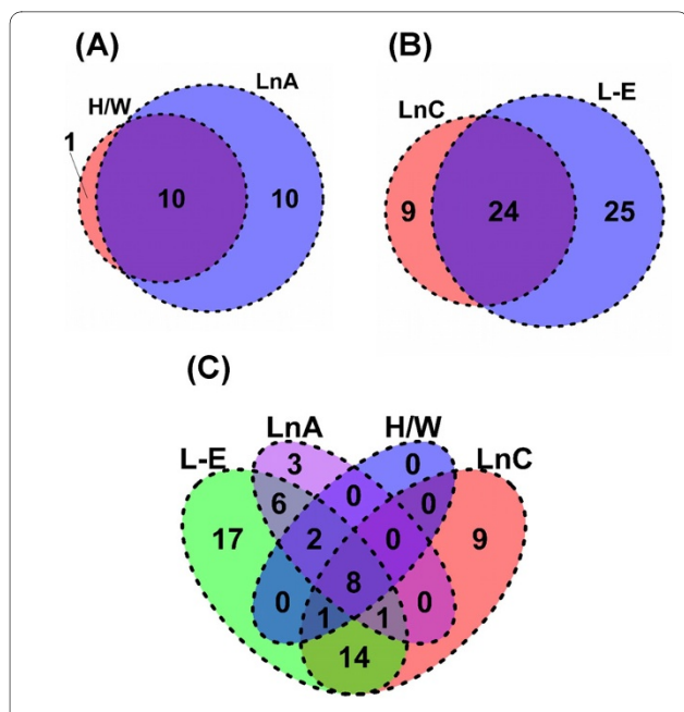
Figure 6 Overlap of functional terms between rat strains/lines. Gene Ontology (GO) analysis was used to determine if different combinations of strains/lines led to alterations in mRNA levels for functionally coherent groups of genes. The gene-lists for each of the four strains/lines were tested for enrichment of each GO category represented on the RAE230A array. False-discovery rates were calculated with 1000 permutations of the dataset using the High-Throughput GoMiner software and a threshold of 5% FDR was applied. The vast majority of GO terms enriched in both the resistant (A) and the sensitive (B) strains/lines overlap. A four-way overlap of all strains/lines shows significant overlap, but also some strain-specific responses (C).
