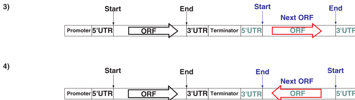
Figure 1 Schematic representation of the definition of Promoters, 5'UTRs, 3'UTRs, and terminators. Two types of promoters appear in parts 1) and 2) Two types of terminators appear in parts 3) and 4). Note that that in cases 1) and 3) the terminator of one gene is the promoter of the next gene. Thus, in the case of terminators, we treated this category separately from the converging case [4].
