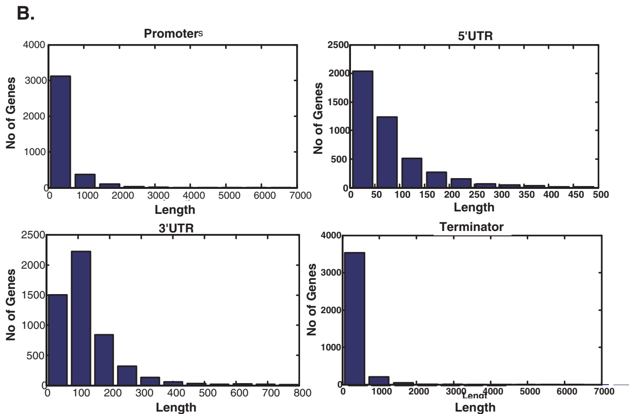
Figure 2 Length distribution of untranslated regions.
