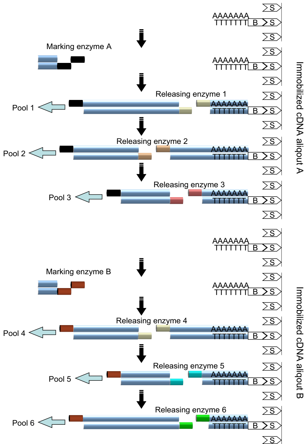
Figure 1 Protocol for sequential digestion cDNA-AFLP. Biotinylated cDNA molecules are bound to streptavidin matrix. Each combination of a marking enzyme (A and B) with a releasing enzyme (one to six) generates a cDNA fragment pool.
