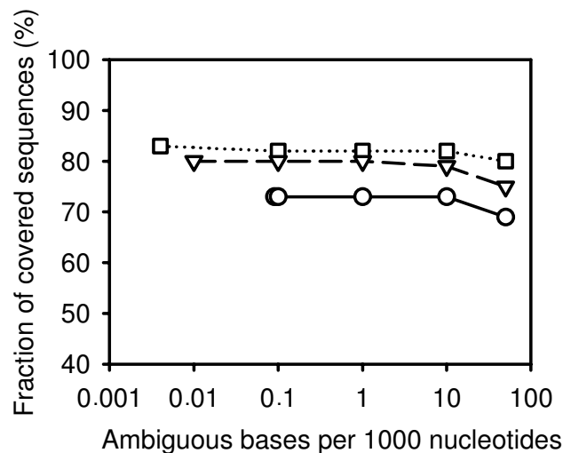
Figure 6 Effect of ambiguous nucleotides on cDNA-AFLP coverage as estimated by simulation. Modified EST sets were generated from RefSeq sequences by labeling different fractions of randomly selected nucleotides as ambiguous using a Perl script. cDNA-AFLP sequential digestion protocol was simulated using the optimal combinations of two marking and three releasing enzymes, and the coverage was plotted against the fraction of ambiguous nucleotides. Squares connected by a dotted line: mouse; triangles connected by a dashed line: human; circles connected by a filled line: Arabidopsis.
