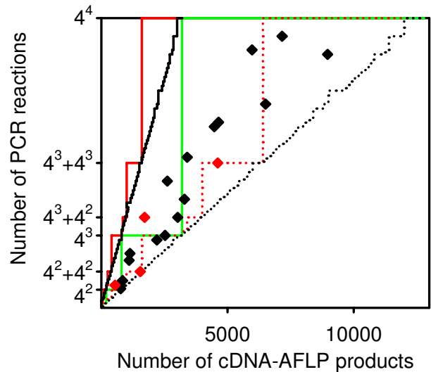
Figure 4 Effect of partitioning fragments into mutually exclusive pools on the total number of PCRs. The lowest number of PCR reactions generating not more than 50 products per PCR on the average is plotted against the number of cDNA-AFLP fragments. PCR is performed either on all fragments in one pool (green line, the number of PCRs equals to the number of primer combinations) or on two (red lines) or six (black lines) mutually exclusive pools of fragments (PCRs are summed up over all pools). For two and six fragment pools (red and black lines, respectively), dotted lines depict the optimal partitioning of fragments (minimum number of PCRs) while full lines depict the least favorable partitioning of fragments (maximum number of PCRs). The results of simulations are shown as diamonds.
