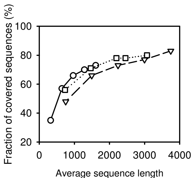
Figure 7 Effect of sequence length on coverage. Modified EST sets were generated from RefSeq sequences by truncating the sequences from the 5' end to a various extent. cDNA-AFLP sequential digestion protocol was simulated using the optimal combinations of two marking and three releasing enzymes. Squares connected by a dotted line: mouse; triangles connected by a dashed line: human; circles connected by a filled line: Arabidopsis .
