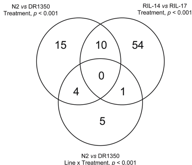
Figure 1 Gene expression in different environments for the four lines. Venn diagram showing the distribution of the number of genes whose expression significantly differs between dauer larva and non-dauer larva-inducing conditions for N2, DR1350, RIL-14 and RIL-17.
