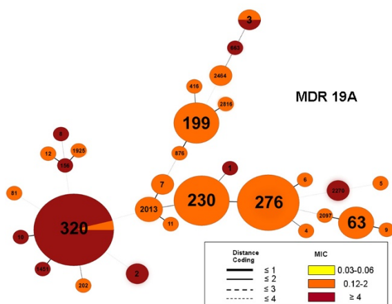
Figure 3 Minimum spanning tree of multi-drug resistant (A) (MDR) serotype 19A ( n = 97 ) using BioNumerics software. A categorical clustering was performed based on multi-locus sequence type (MLST). Sequence types sharing the maximum number of single-locus variants were connected first. Each circle represents a sequence type (ST) the size of which is proportional to the number of isolates within that particular ST. Colors within circles indicate the minimum inhibitory concentration (MIC) ranges for penicillin. Relationships between the STs are depicted by the lines connecting the STs and the relative lengths of the branches linking them. Distance coding enumerates the number of differences at a given MLST locus. A distance coding of greater than 2 implies a different clonal complex. Angles of the line connections and the overlapping circles have no significance.
