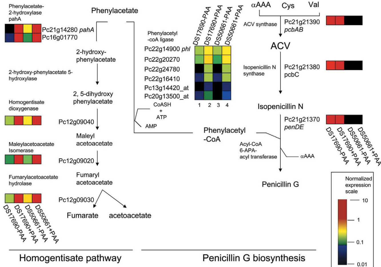
Figure 6 Detoxification of phenylacetic acid via incorporation into penicillinG or the homogentisate pathway. Those genes (putatively) related to penicillin, biosynthesis and phenylacetate catabolism are depicted. Total RNA was obtained from P. chrysogenum strains DS17690 and DS50661, grown in the presence and absence of phenylacetic acid (PAA) in independent glucose-chemostat cultures at D = 0.03 h -1 and hybridized to Affymetrix GeneChip® microarrays. The color bar indicates the range of the mean normalized transcript level value per gene. αAAA: α-aminoadipate, Cys: cysteine and Val: valine.
