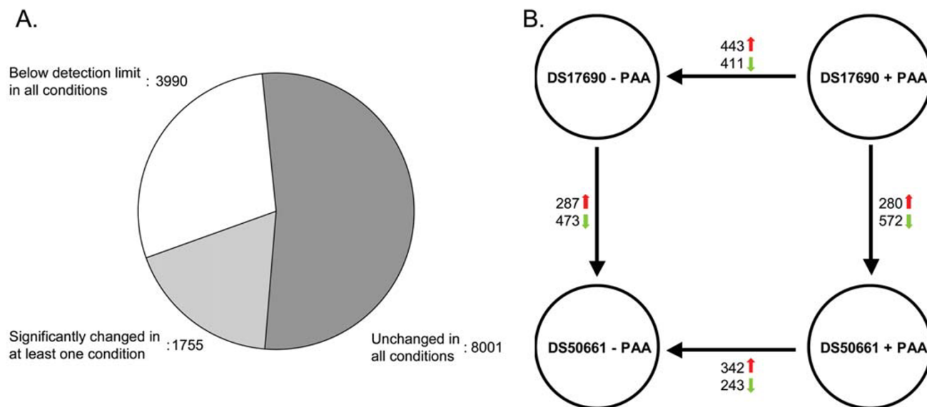
Figure 2 Global gene expression response of DS17690 and DS50661 strains to the presence and absence of PAA. Total RNA was obtained from P. chrysogenum strains DS17690 and DS50661, grown in the presence and absence of phenylacetic acid (PAA) in independent glucose-limited chemostat cultures at D = 0.03 \text{ h}^{-1} and hybridized to Affymetrix GeneChip® microarrays. A: Pie chart of overall transcript differences of the DS50661 and DS17690 strains grown in the absence and presence of PAA. B: Results of the pairwise comparisons of the two strains and the two conditions. Red arrows indicate genes with a higher transcript level in the respective pairwise comparison, green arrows indicate genes with a lower transcript level.
