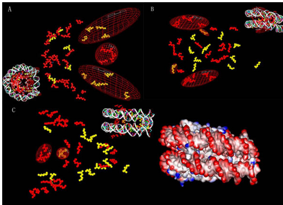
Figure 2 3D location of acetylability related lysine groups. The view angles are labeled as A, B and C. The balls in yellow represent the acetylable lysine, while red for the un-acetylable in training set. The wired ellipsoids are 3D regions related to acetylability. The lysine only and whole nucleosome parts are contained in all three views. An additional surface colored by electronically potential is added to C on the right side.
