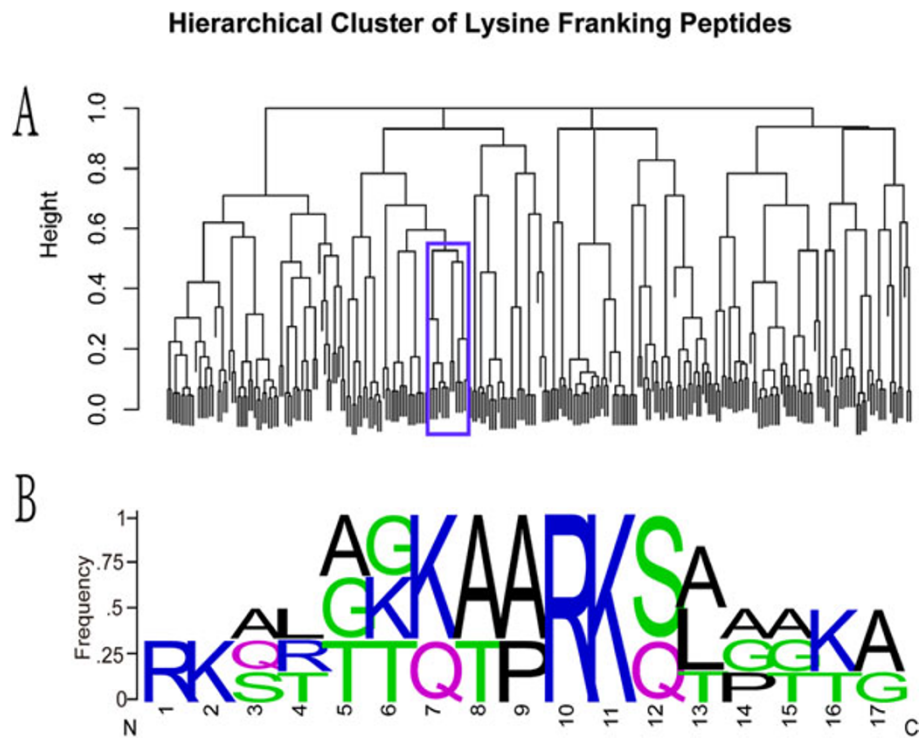
Figure 1 Hierarchical Cluster of Lysine Franking Peptides and Cluster peptide Pattern Graph A represents the hierarchical cluster dendrogram of all the peptides of human and A. thaliana . The subtree in blue rectangle contains H3K4, H3K9, H3K14, H3K18, H3K23 and H3K27, and graph B is the related sequence pattern in WebLog.
