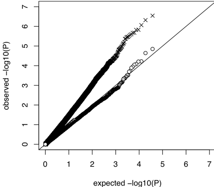
Figure 10 Quantile - quantile plot for protein yield under the null distribution from method MIX (X) and MIXStrat (O).
