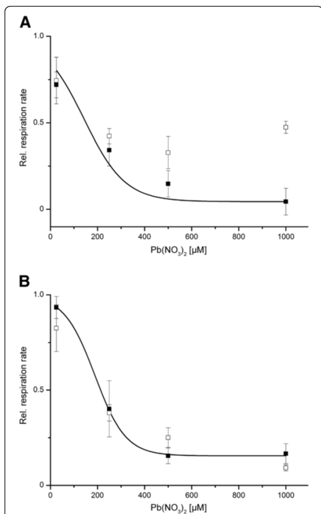
Figure 4 Relative respiration rates of Arthrobacter sp. Rue61a and A. aurescens TC1 in response to Pb 2+ . Arthrobacter sp. Rue61a (A) and A. aurescens TC1 (B) were cultivated in LB medium in the presence and absence of 10 μM Pb(NO 3 ) 2 . Cells were resuspended in 10 mM MES buffer, pH 6.5, and respiration rates of cells pre-grown in the presence of Pb(NO 3 ) 2 (empty squares) and of cells grown in the absence of Pb 2+ (filled squares) were measured at different concentrations of Pb(NO 3 ) 2 . The relative respiration rate is the ratio of the ΔO 2 after and prior to Pb(NO 3 ) 2 injection. Data represent mean values ±SD (standard deviations) from three independent experiments. The continuous lines represent fits of a dose-response equation to the data of the LB-grown cells.
