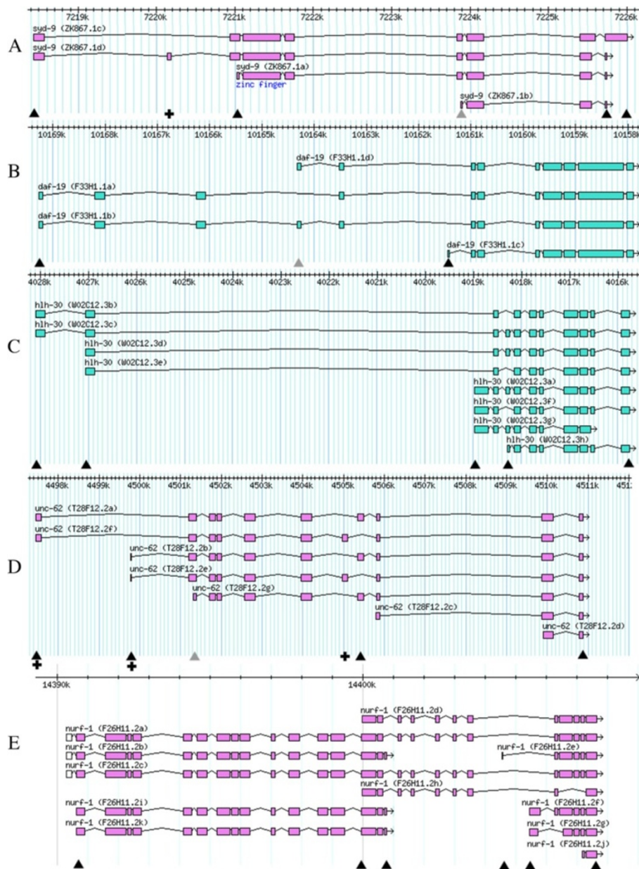
Figure 6 Gene models for assayed genes with multiple mechanisms of alternative transcript generation. A. syd-9 . B. daf-19 . C. hlh-30 . D. unc-62 . E. nurf-1 . The molecular gene names are included in brackets after the genetic gene name, with the additional final letter (a/b/c etc.) distinguishing the transcripts encoding distinct isoforms. The triangles indicate positions of gfp insertion used to tag expression for different transcripts. The grey triangle indicates that gfp was inserted with an extra nucleotide upstream to disrupt the translational reading frame, and therefore reporter expression, for other transcripts starting further upstream. The crosses indicate where translational reading frames of protein-coding regions were disrupted by the insertion of single base pairs to eliminate reporter expression arising from particular transcripts for fusion genes with gfp inserted at the end of the protein coding region. For nurf-1 , the first exons (white) of transcripts a, b and c were included in WS190, but not WS230. The scale bar in each panel is in base pairs along the respective chromosome.
