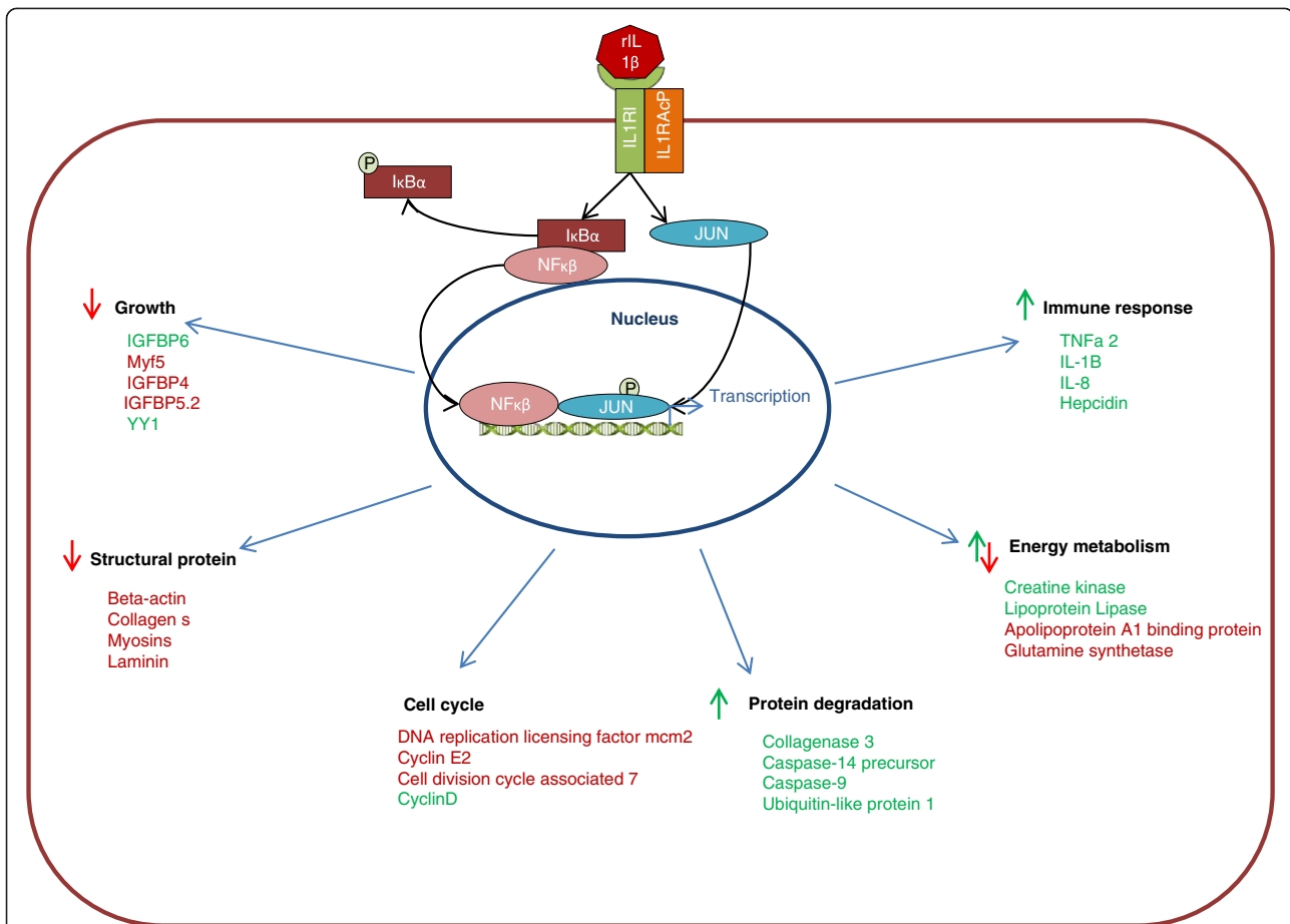
Figure 5 Model of the proposed actions of rIL-1β on gene expression and physiology of muscle cells in vitro . rIL-1β is recognised by its receptor and an accessory protein, this then sets off a signal cascade resulting in the activation of NFκβ and JUN which in turn result in changes in gene expression and physiology. The proposed changes in physiology are shown in black. Green arrows show a positive effect on this aspect of physiology and red arrows show a negative effect. A sample of genes related to each aspect of physiology is shown in either red (up regulation) or green (down regulation).
