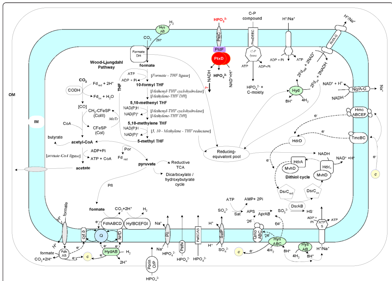
Figure 3 Pathways of dissimilatory electron flow, autotrophic CO 2 assimilation and phosphorus metabolism in D. phosphitoxidans . Arrows indicate established metabolic paths; dashed arrows indicate hypothetical electron flows. For the sake of simplicity, oxidation pathways for organic substrates are not shown. Phosphonate dehydrogenase is shown in red; the NAD(P)-dependent epimerase/dehydratase PtdF is shown in purple; high-affinity symporters are shown in grey; hydrogenases are shown in green and the soluble cytochromes are shown in yellow.
