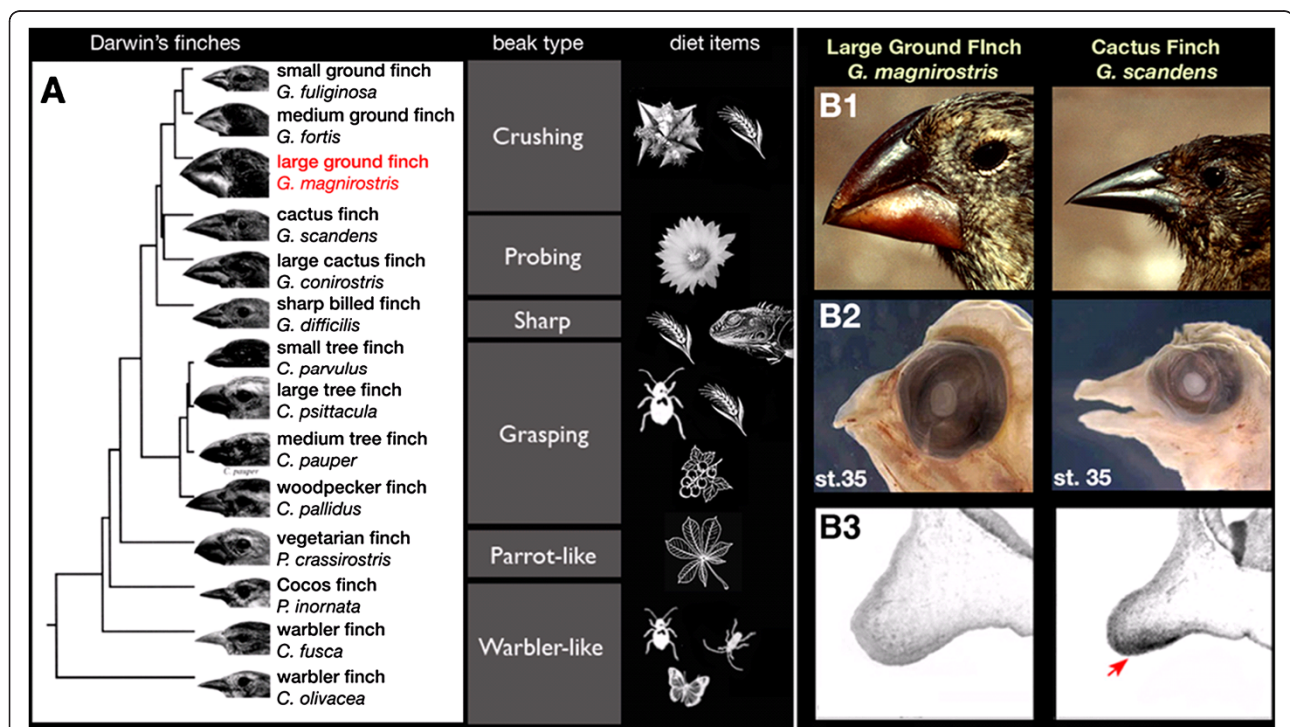
Figure 1 Evolutionary mechanisms for beak shape diversity in Darwin’s finches (Thraupidae, Passeriformes). (A) Molecular phylogeny of 14 species of Darwin’s finches shows a range of beak shapes in this group of birds. These species have beaks of different shapes that allow them to feed on many different diets: insects, seeds, berries, and young leaves. Species are numbered as follows: small ground finch Geospiza fuliginosa ; medium ground finch G. fortis ; large ground finch G. magnirostris ; cactus finch G. scandens ; large cactus finch G. conirostris ; sharp-billed finch G. difficilis ; small tree finch C. parvulus ; large tree finch Camarhynchus psittacula ; medium tree finch C. pauper ; woodpecker finch C. pallidus ; vegetarian finch Platyspiza crassirostris ; Cocos finch Pinaroloxias inornata ; warbler finch Certhidea fusca ; warbler finch C. olivacea (phylogeny from [5]). (B1) Large ground finch (left) has a very deep and broad bill adapted to crack hard and large seeds, while the cactus finch (right) has an elongated and pointy beak for probing cactus flowers and fruits. (B2) Geospiza finch bills develop their distinct shapes during embryogenesis and are apparent upon hatching (mid-development stage 35 embryos are shown from Abzhanov et al. [12]). (B3) The cactus finch-specific expression of CaM was validated by in situ hybridization after it was identified as a candidate by a microarray screen [14].
