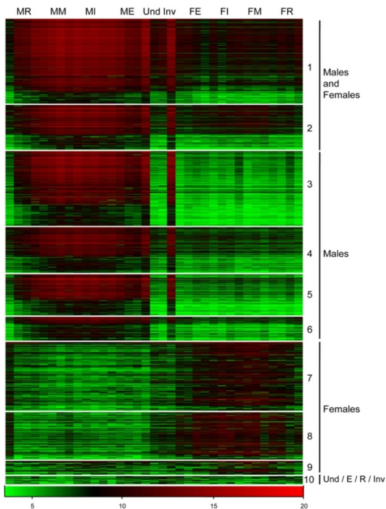
Figure 6 Heat map of contigs differentially expressed between the ten different gonadic categories of P. margaritifera . Clusters of the 1,993 differentially expressed contigs (rows) were obtained with K-means clustering using Spearman's correlation. Contigs showing similar expression profiles on all samples (columns) clustered together. (M/F)E: male/female at early stage; (M/F)I: male/female at intermediate stage; (M/F)M: male/female at mature stage; (M/F)R: male/female at stage of regression; Inv: gonads in sexual inversion; and Und: gonad sex is undetermined. Four main expression profiles are identified: Males and Females (genes expressed in both sexes with expression changing over the course of gametogenesis, 561 contigs); Males (genes highly expressed in males with expression increasing over the course of spermatogenesis, 815 contigs); Females (genes highly expressed in females with expression increasing over the course of oogenesis, 574 contigs); and genes more expressed in undetermined, early, regressed gonads and in gonads in sexual inversion (43 contigs). Color represents the normalized expression after variance-stabilizing transformation (DESeq). Expression levels are depicted with a color scale, in which shades of red represent higher expression and shades of green represent lower expression.
