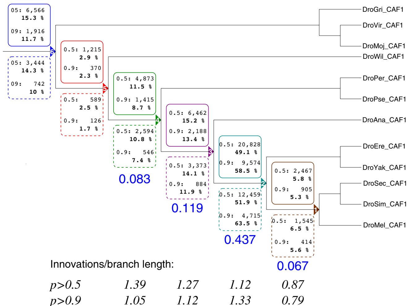
Figure 5 Phylogenetic distribution of ncRNA candidates. The tree only represents the topology and is not drawn to scale. Branch lengths are indicated below by large numbers in sans serif font, measured in terms of substitutions per site for 4-fold degenerated sites. For each branch we mark the number of RNAz hits for p > 0.5 and p > 0.9 , respectively above the branch leading to the last common ancestor (LCA) of the sequences in the corresponding input alignment (full boxes). Below the branches we indicate the corresponding numbers for the "gentle" control screen. Below the tree the ratio of the fraction of newly appearing RNAz hits and the branch length is given, indicating little variation in the "innovation rate". Since the original tree is unrooted without an outgroup, no data are available for the branch separating Sophophora from the rest. The number of RNAz hits listed in the tree is smaller than the total number of RNAz hits because we only considered sequences present in all single windows of an RNAz hit here.
