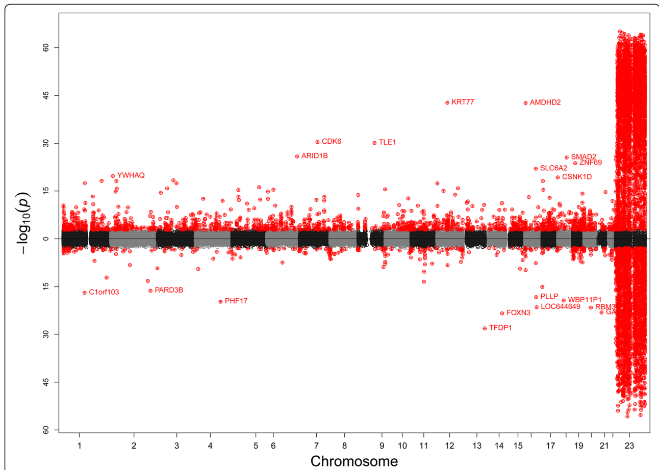
Fig. 1 Manhattan plot for association between child sex and DNA methylation at all 450 K CpGs, adjusting for batch and cell composition by differential cell count (DCC). Associations where methylation was higher for girls relative to boys are plotted above the x-axis, while those with decreased methylation are plotted below. CpGs meeting FDR multiple testing threshold of ( P < 0.05 ) shown in red
