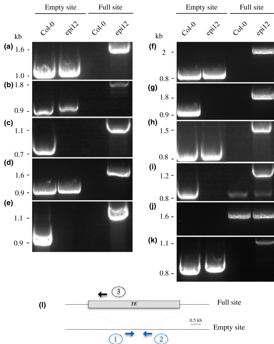
Fig. 3 Validation of EVD insertions in epiRIL12 detected by MinION. PCR detection of EVD insertion polymorphism for neo-insertion 1 to 9 (a to i), the native copy of EVD on chromosome 5 as control (j), and the neoinsertion of CAC1 (k). l : schematic illustration of RBIP primer design. primers 1 and 2 are designed to detect empty sites and primers 1 and 3 (sense insertion) or 3 and 2 (antisense insertion) are designed to detect full sites
